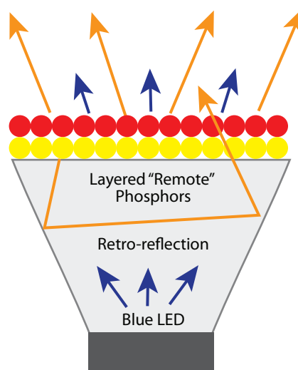
Figure 8 — Two strategies for increasing the efficacy of LEDs are to layer the phosphors in order of increasing emitted wavelength, and use optics to retro-reflect some of the scattered light out of the LED. By keeping the phosphors away from the hot LED chip, the characteristics should last longer.
